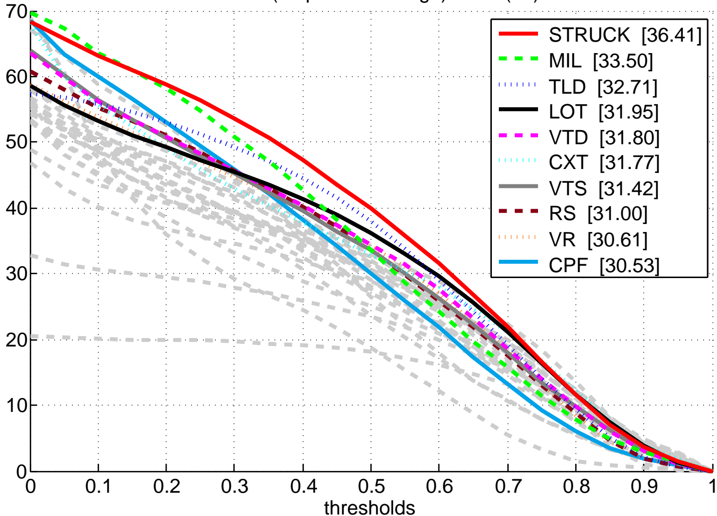
TRE50 (sequence average) – OV (11)
