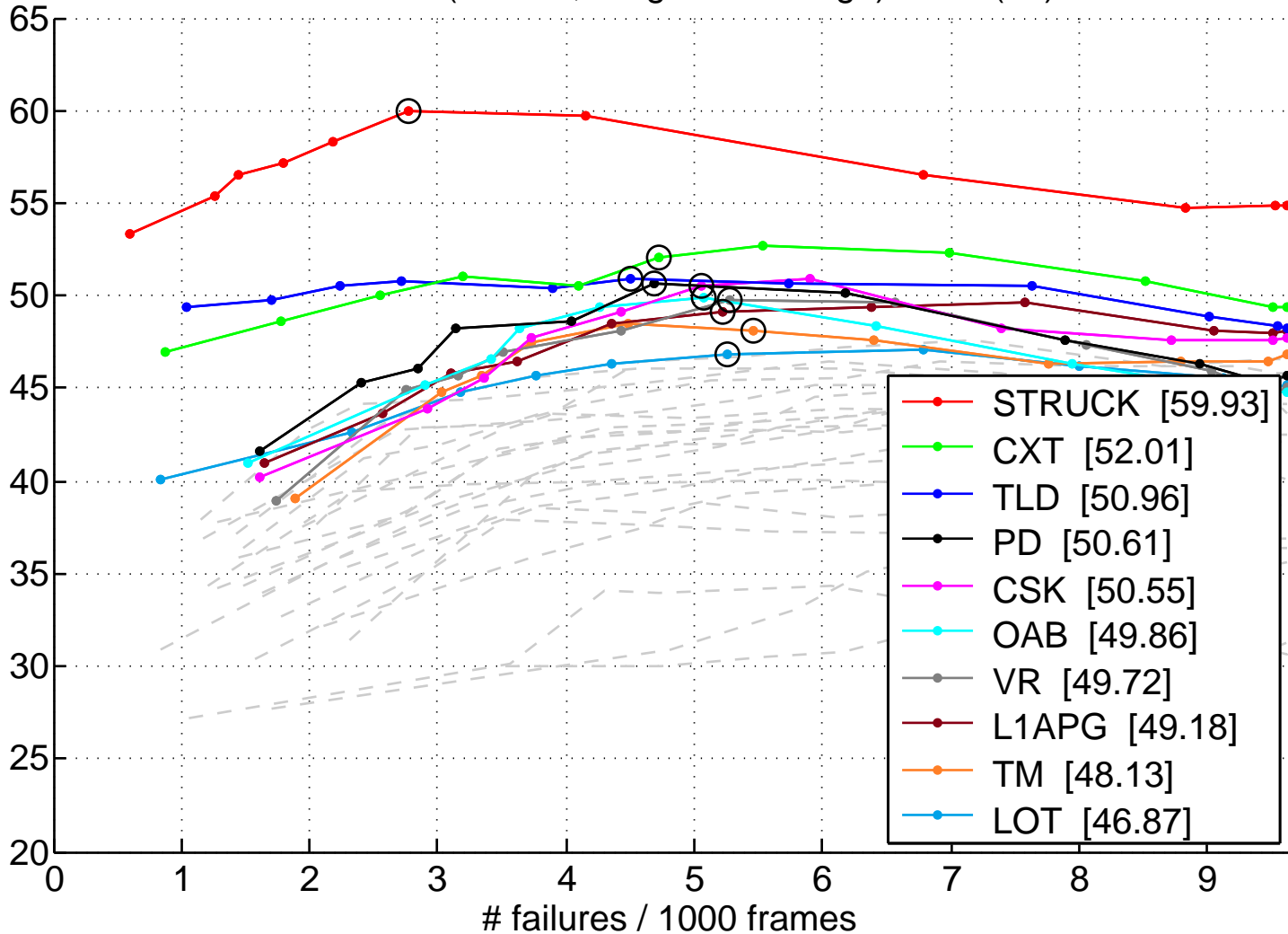
SRER 50 (win=90, weighted average) – MB (19)
