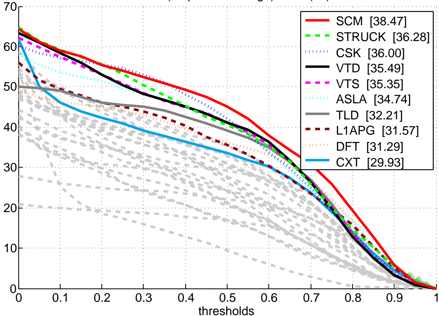
OPE50 (sequence average) – BC (20)
