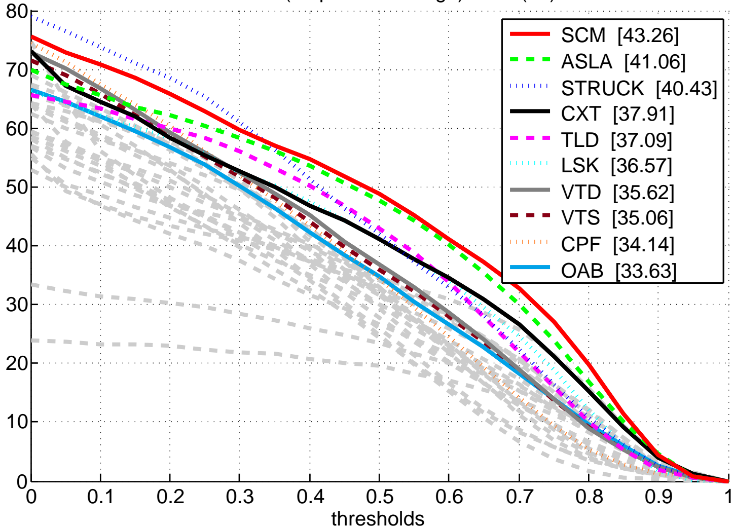
OPE100 (sequence average) – SV (64)
